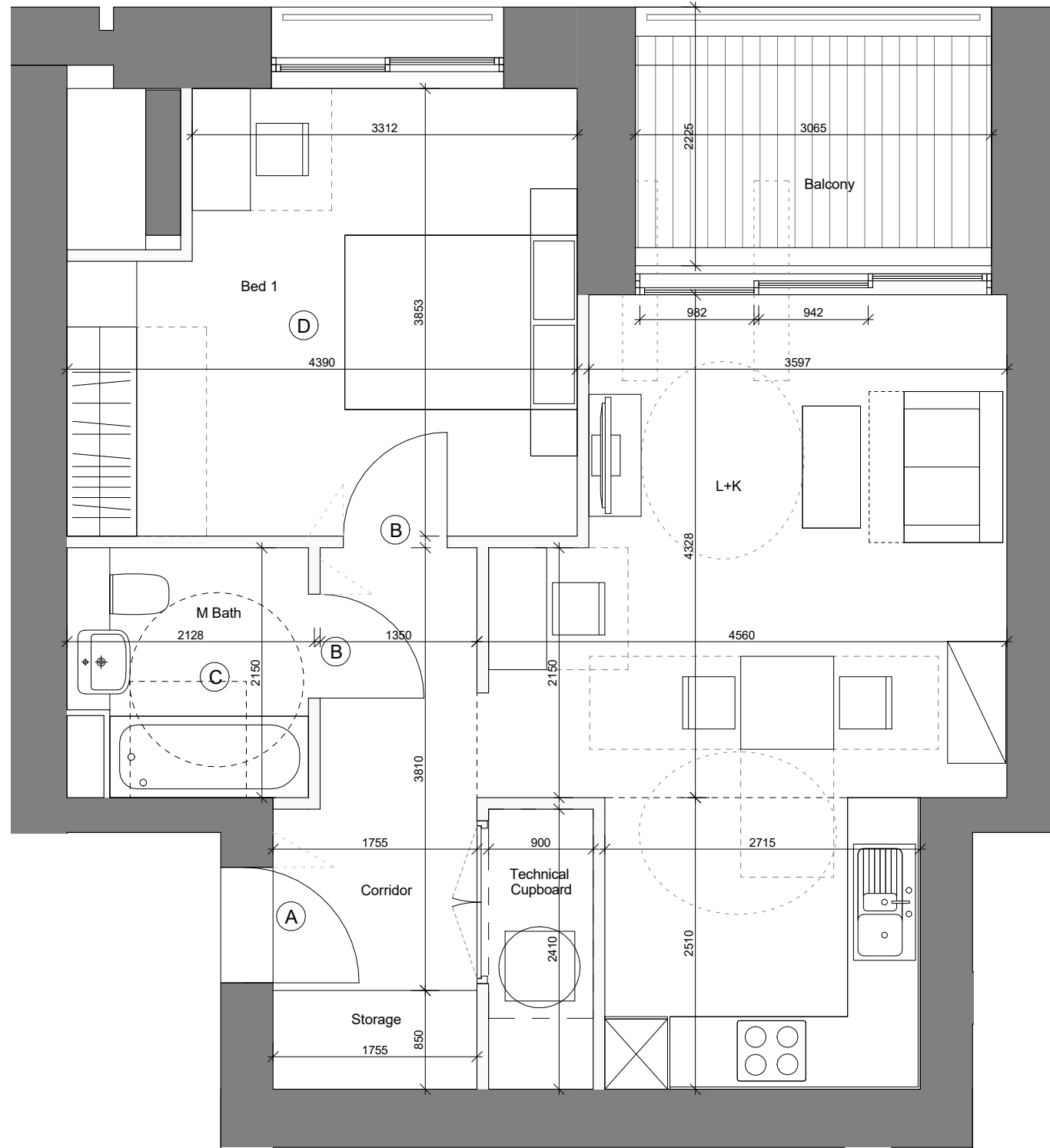
K2 01 First Floor 1B-2P-04
