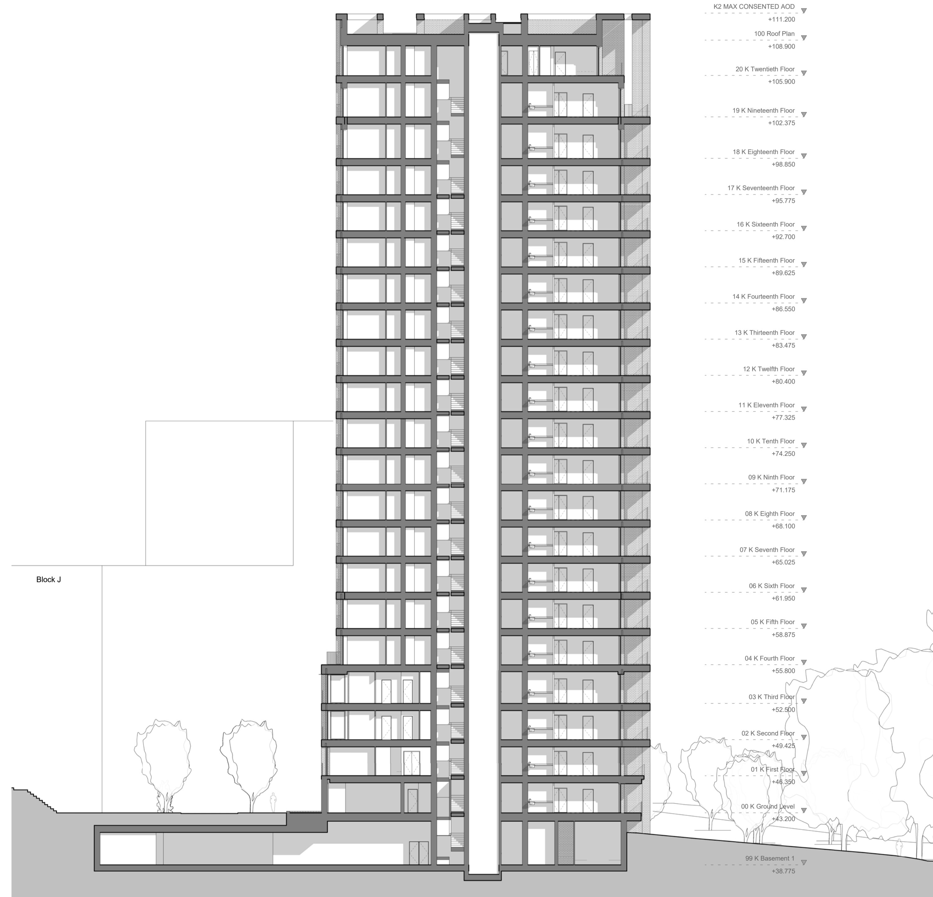
1 Section B-B1 1:200
