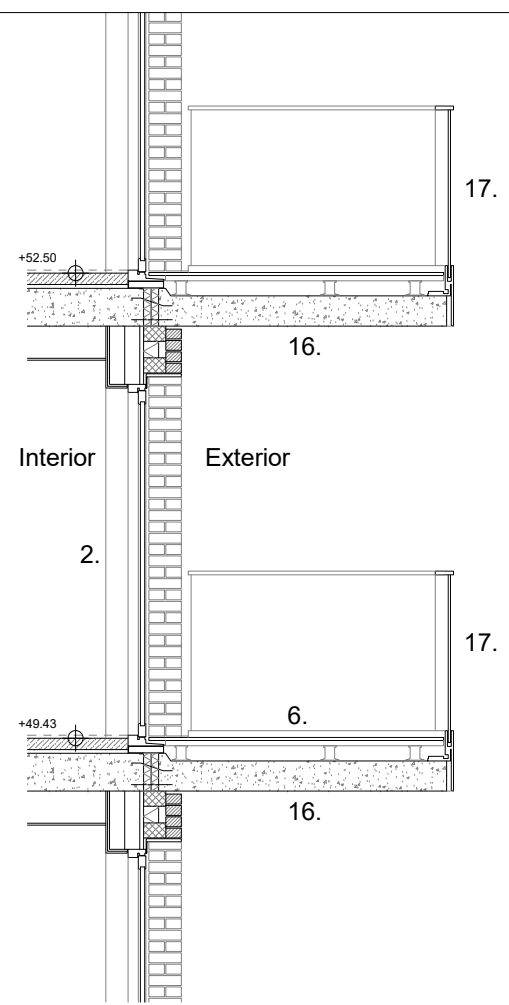
2 Section 1 - Baystudy 4
