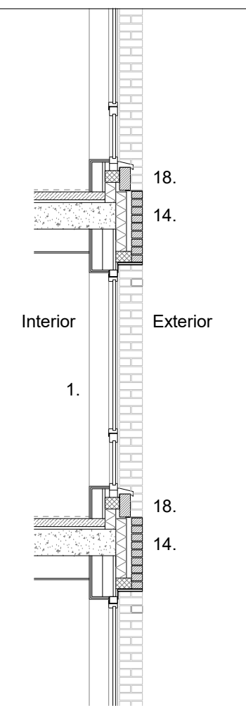
6 Section 3 - Baystudy 4
